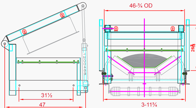
Magnetic Release of Tramp Iron Position
