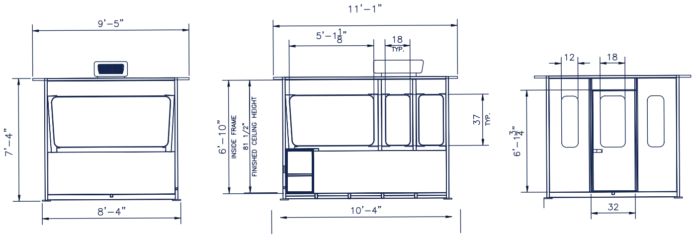
8'x10' Stationary Control Tower General Arrangement
