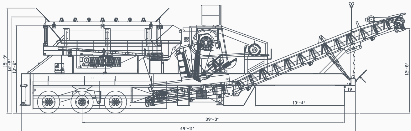
ELRUS 2442 Jaw Plant General Arrangement
