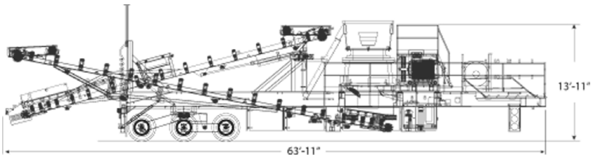
Travel Weights & Dimensions Length: 63'-11" Axle weight: 58,422 lbs (26,500 kg) Width: 11'-9" Pin Weight (Including truck): 38,490 lbs (17,460kg) Height: 13'-11"
